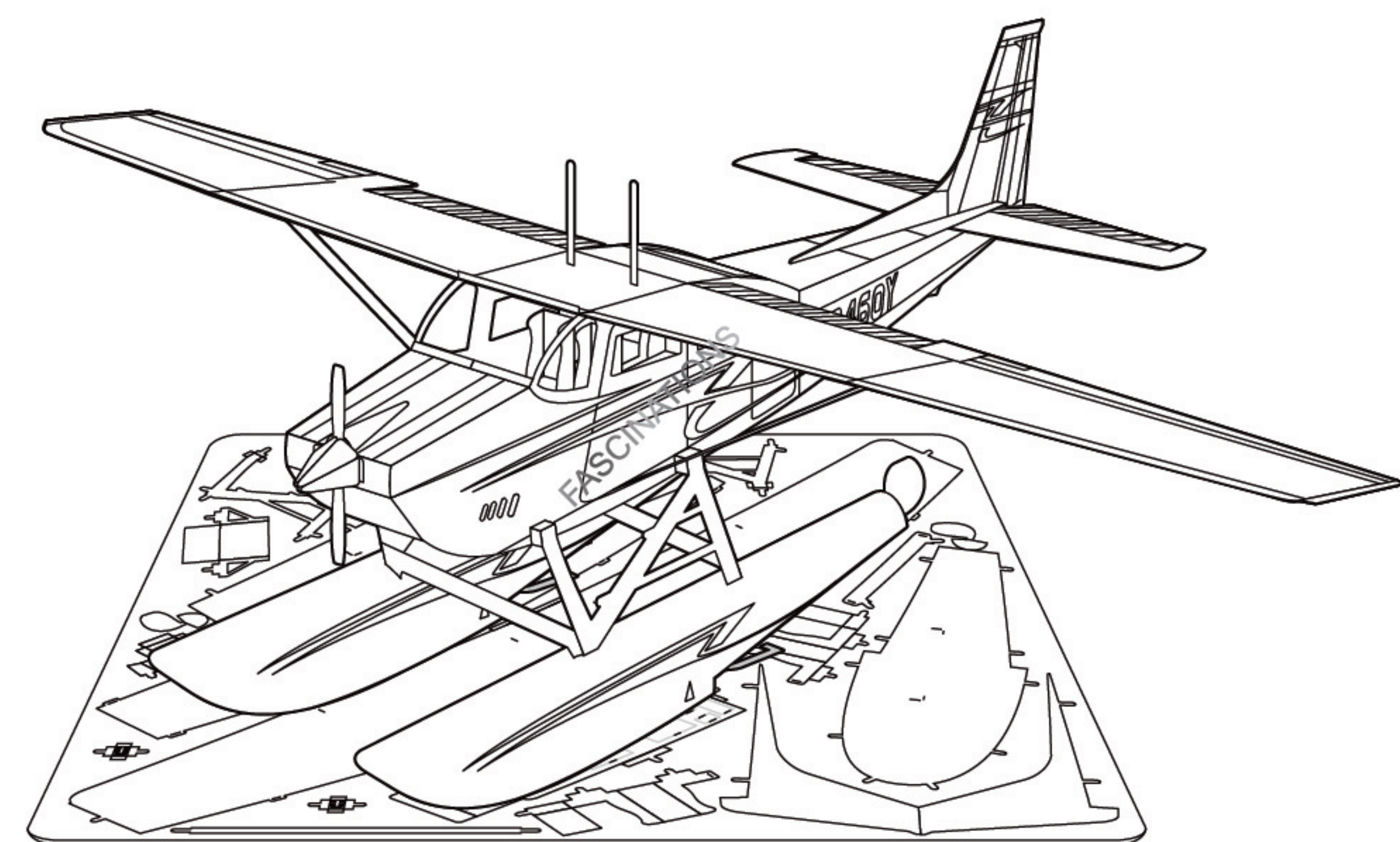
Cessna 182 Skylane Item No. MMS111
